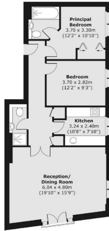
Second Floor
